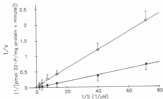
FIGURE 1: Double-reciprocal plot of the dephosphorylation rate of the 1142–1153 peptide. Cytosolic and particulate PTPase fractions were incubated with various concentrations of 32 P-labeled 1142–1153 peptide for 5 min at 30 °C. After precipitation of proteins in 10% TCA, free [ 32 P]P i was extracted and counted. Open and filled circles represent the cytosolic and particulate PTPase activity, respectively. The data are expressed as the mean \pm SEM of triplicates; similar results were obtained in three separate experiments.
